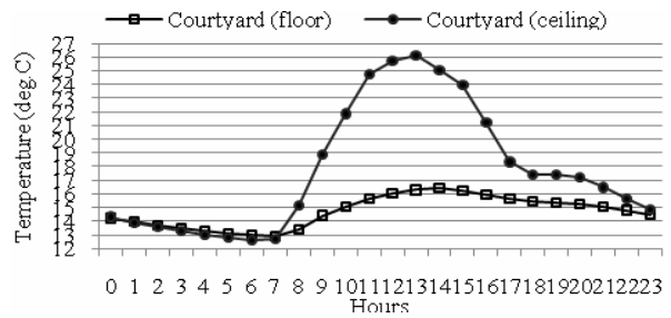
Fig. 11 Mean temperatures of Auckland ‘wind-rain’ house’ courtyard
