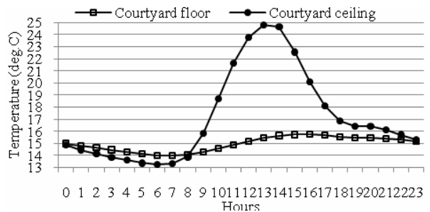
Fig. 12 Mean temperatures of Wellington ‘wind-rain’ house’ courtyard
