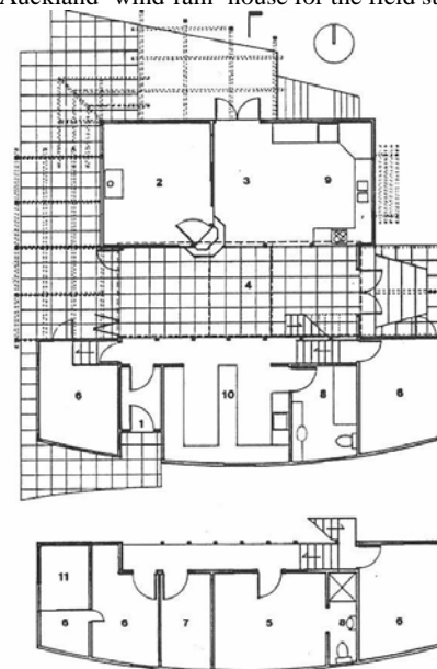
Fig. 2 The Auckland ‘wind-rain’ house plans
