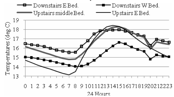
Fig. 13 Mean temperatures of upstairs and downstairs bedrooms
