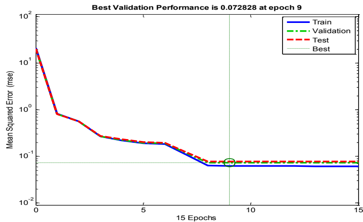
Figure 2. The best validation performance is 0.072828 at epoch 9 with seven input variables (Tmax, Tmin, P, RH, SZA, Az, Ra).
