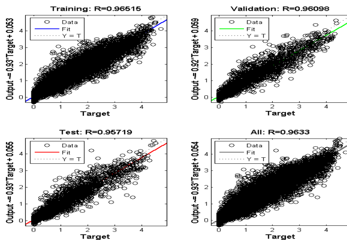
Figure 3. Regression analysis of the network outputs with respect to targets for training, validation and test sets.
