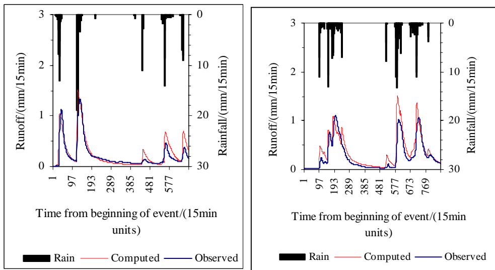
Figure 10: Observed and GA-optimised Tank model estimated hydrographs for validation events for Shek Pi Tau
