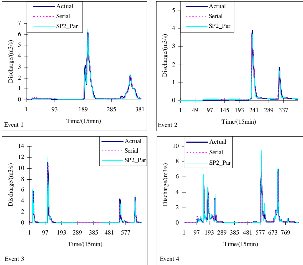
Figure 7: Actual and calibrated Tank model outputs using Serial and Parallel GA.
