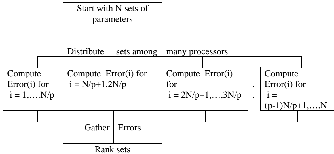
Figure 5 : Parallel Computation of the Objective Function (Error) with p processors
