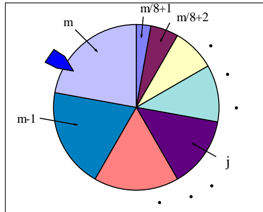
Figure 3: Probability of the reproducing structures
