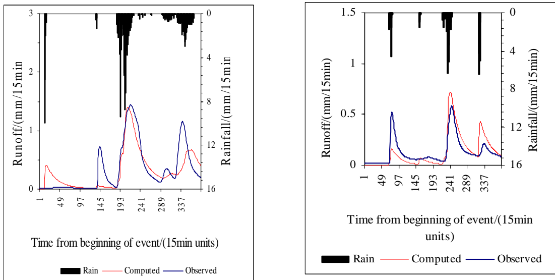
Figure 9: Observed and GA-optimised Tank model estimated hydrographs for calibration events for Shek Pi Tau
