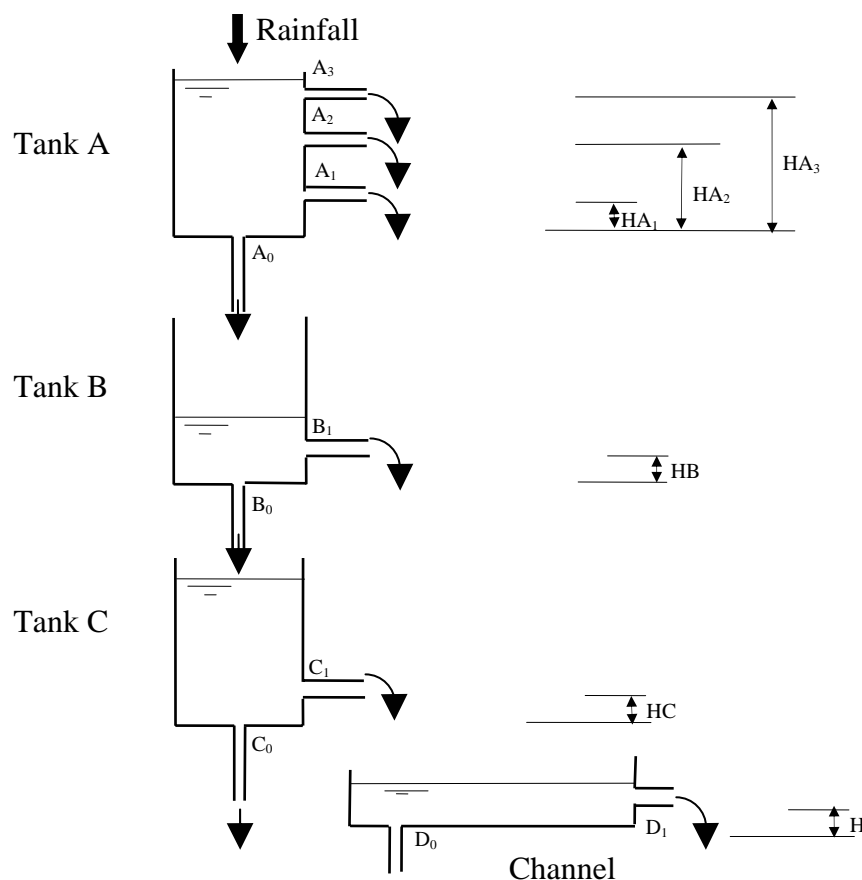
Figure 1: Representation of Tank Model
