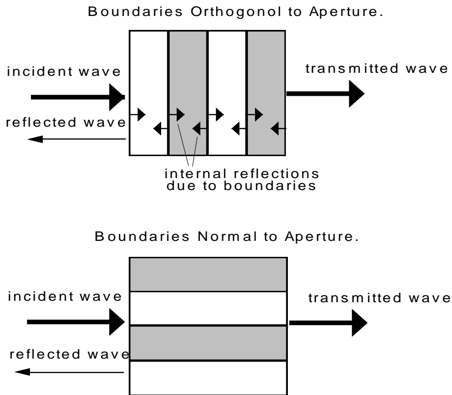
Figure 2. EW/LW layering
