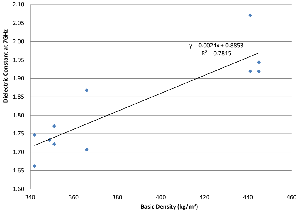
Figure 6. Measured Dielectric constant at 7GHz versus Basic Density
