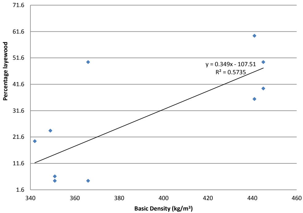
Figure 7. Percentage Latewood versus Basic Density
