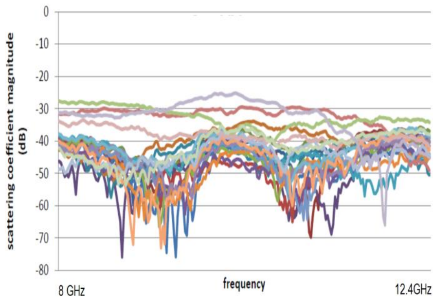
Figure 10. Scatter coefficient S_{13} magnitudes vs. frequency ( 8 to 12.4 GHz range) for twenty two samples, measured in nominal vertical polarization
