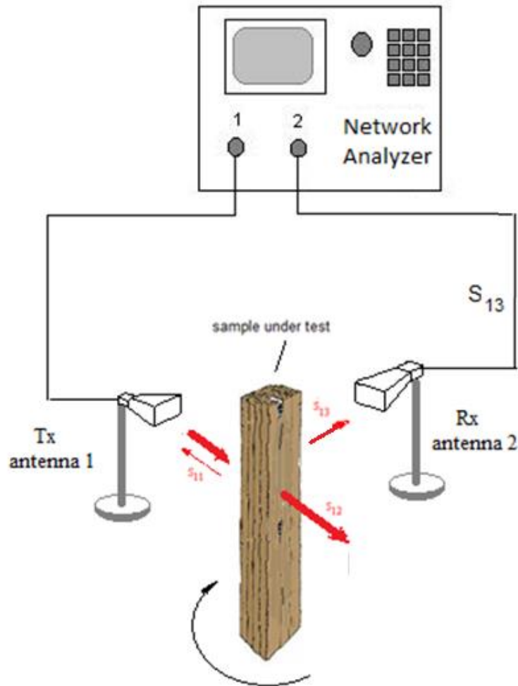
Figure 9. Measurement setup
