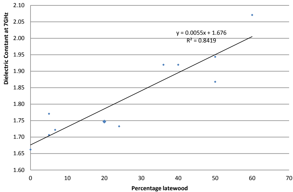
Figure 5. Measured Dielectric constant at 7GHz versus percentage late wood in the sample
