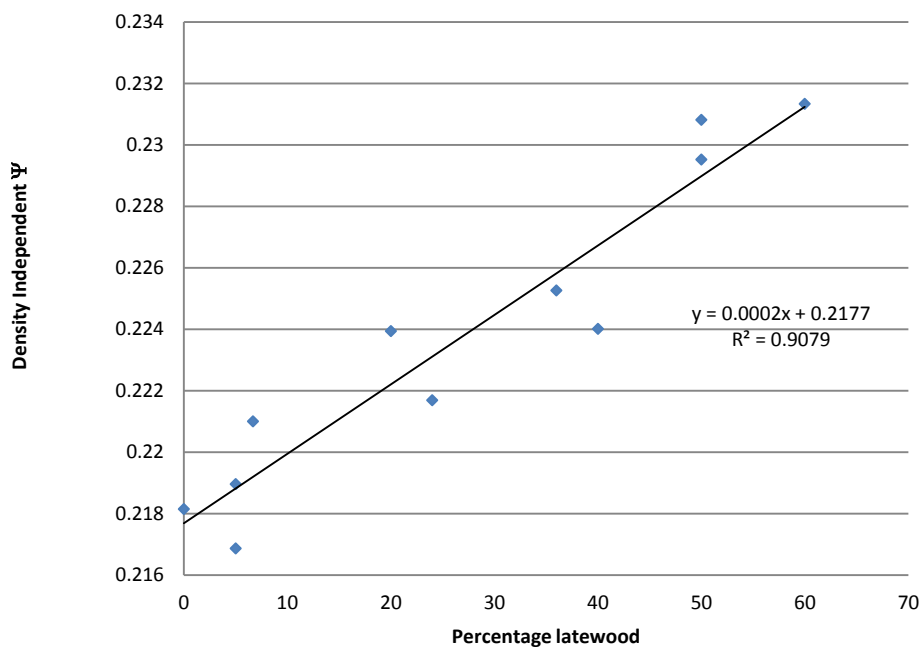
Figure 8. Density Independent Factor at 7GHz versus Percentage Late wood
