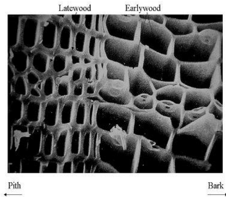
Figure 1. Microscopic image of Earlywood Latewood Structure
