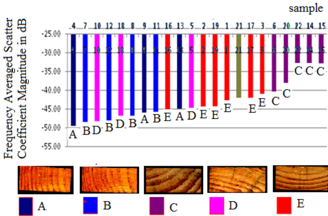
Figure 12. Frequency Averaged Scatter Coefficient Magnitudes and samples grouped by the annual ring pattern
