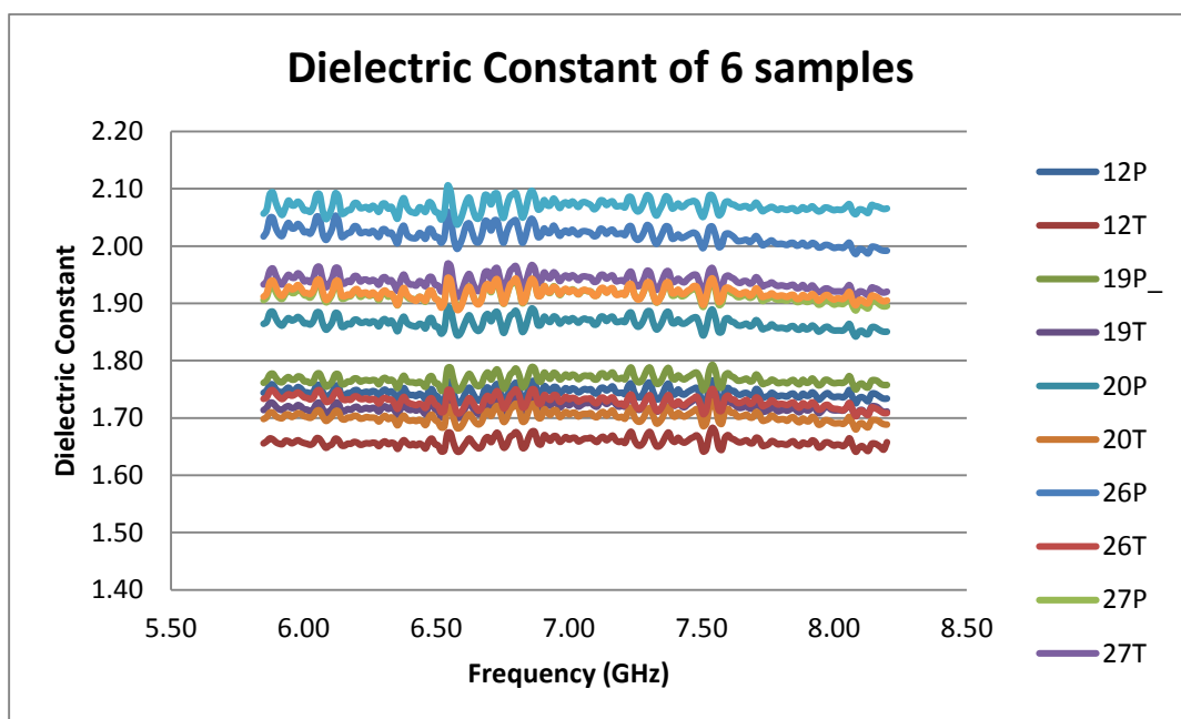
Figure 4. Dielectric constant versus frequency for 6 samples both Parallel and Tangential to
