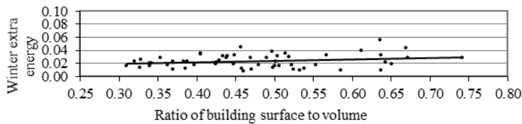
Figure 2. Winter extra energy and ratios of building surface to volume of sample schools
