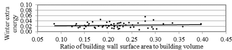
Figure 4. Winter extra energy and ratio of building wall surface area to building volume
