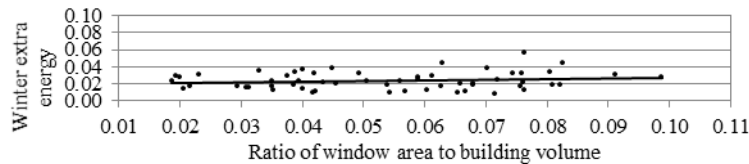
Figure 6. Winter extra energy and ratio of window area to building volume
