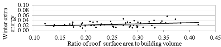
Figure 3. Winter extra energy and ratio of building roof surface area to building volume
