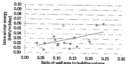
Fig. 11 Winter energy and ratios of wall area to building volume
