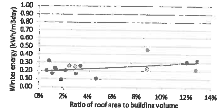
Fig. 25 Winter energy and ratios of roof area to building volume
