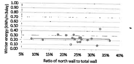
Fig. 14 Winter energy and ratios of north wall to total wall area
