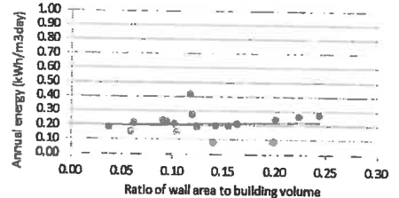
Fig. 10 Annual energy and ratios of wall area to building volume
