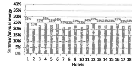
Fig. 3 Ratio of total summer to annual energy consumptions
