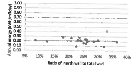
Fig. 13 Annual energy and ratios of north wall to total wall area
