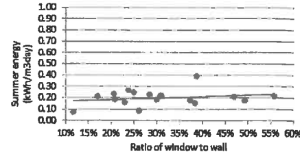
Fig. 21 Summer energy and ratio of window to wall area
